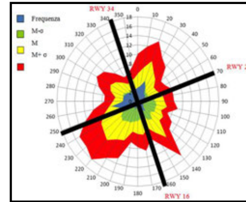
Meteorological Analysis ( wind diagram)
