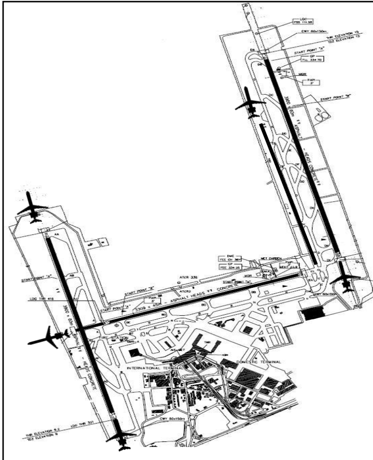
Rome Fiumicino – Short Term Development Plan : new 4 th Runway Project (16C-34C).
